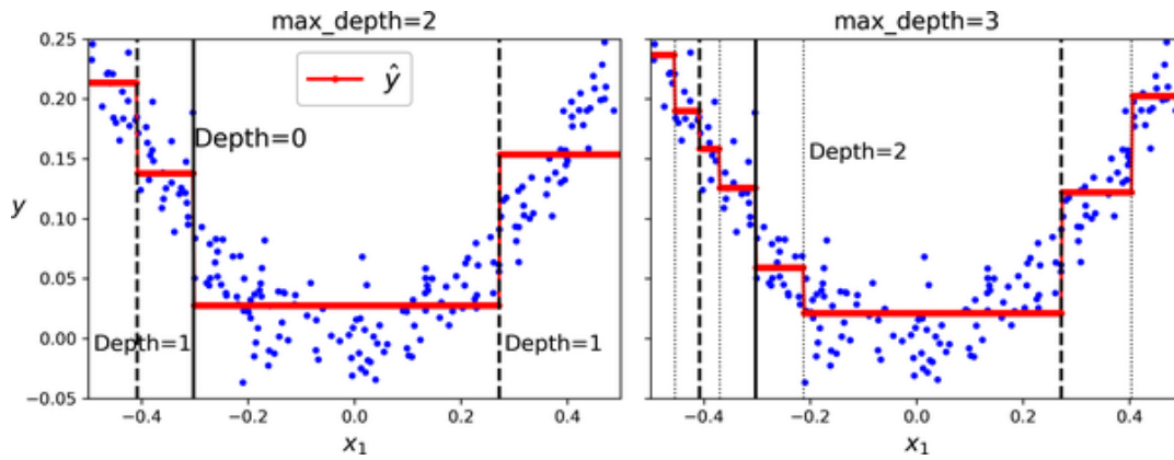
Figure 6-5. Predictions of two decision tree regression models
